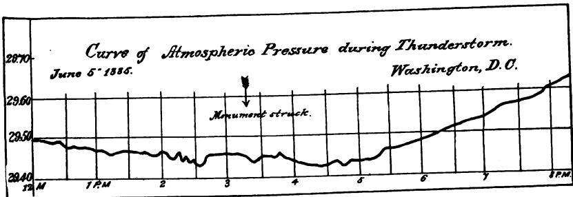
Fig. 8. Curve of barometric pressure.
